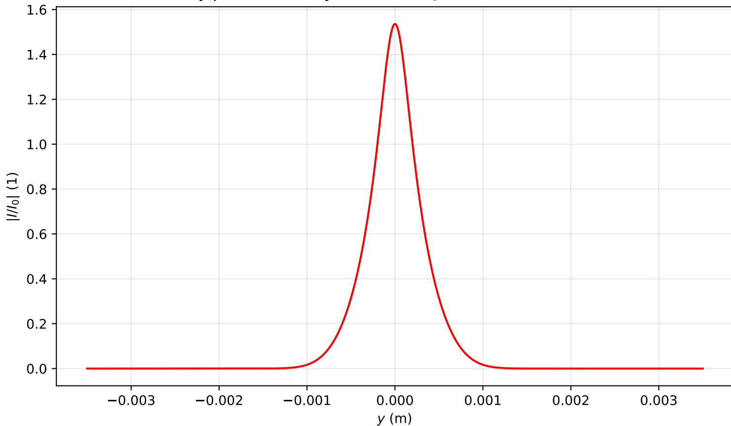
Intensity profile I(x=0, y, z=0.239)/I_0 , \text{Pin}=6.0\text{Pcr} , artificial time
